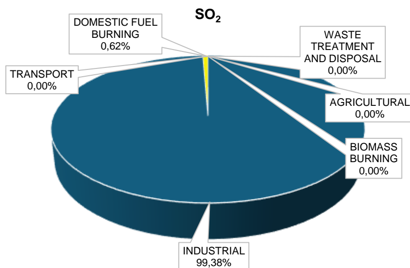
Figure 6-7: The contribution of emissions by sector of sulphur dioxide in the Bitou LM.
