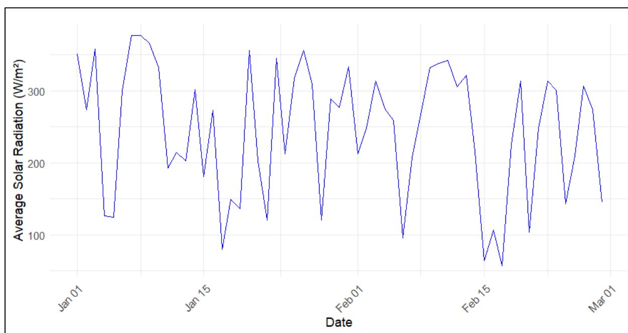
Figure 4-7: Solar radiation in the GRDM for the Summer months (excluding December) for 2023.
