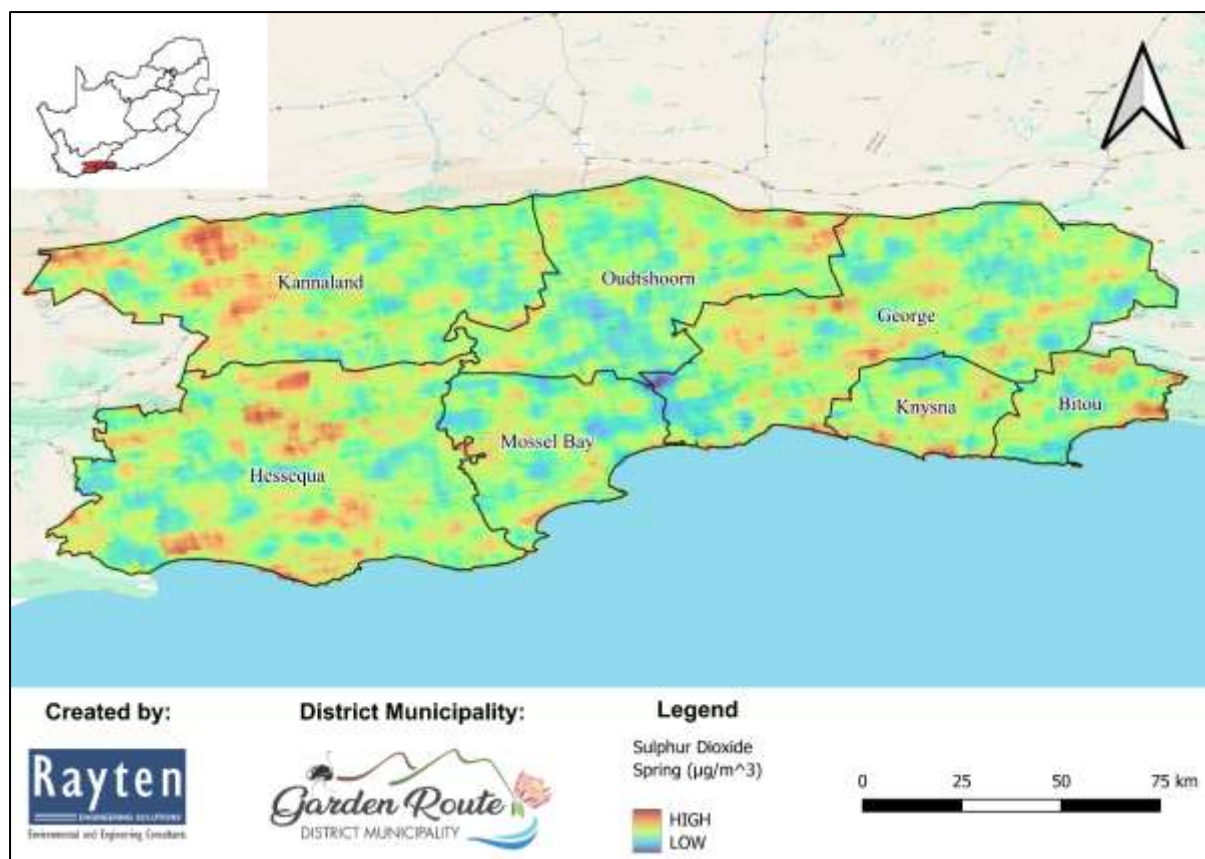
Figure 5-9: Air quality report map indicating concentrations of sulphur dioxide ( \mu\text{g}/\text{m}^3 ) in spring in the GRDM for each season.
