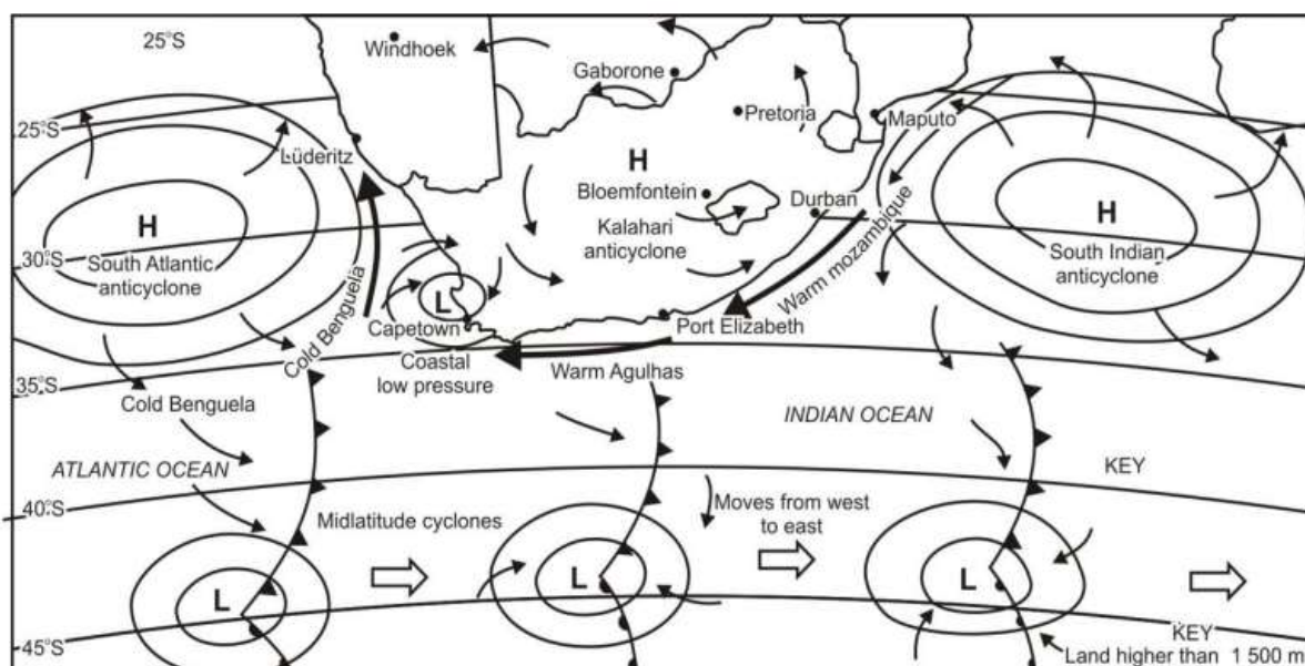
Figure 4-1: Air circulation in and around South-Africa (www.learnxtra.co.za: Section three: Factors that influence weather in South Africa).
