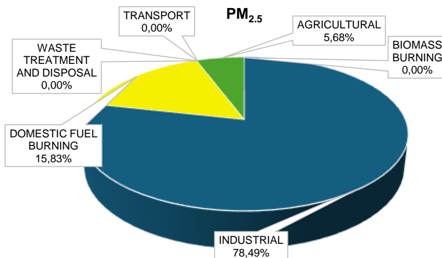
Figure 6-6: The contribution of emissions by sector of particulate matter with a diameter of 2.5 micrometres or less in the Bitou LM.
