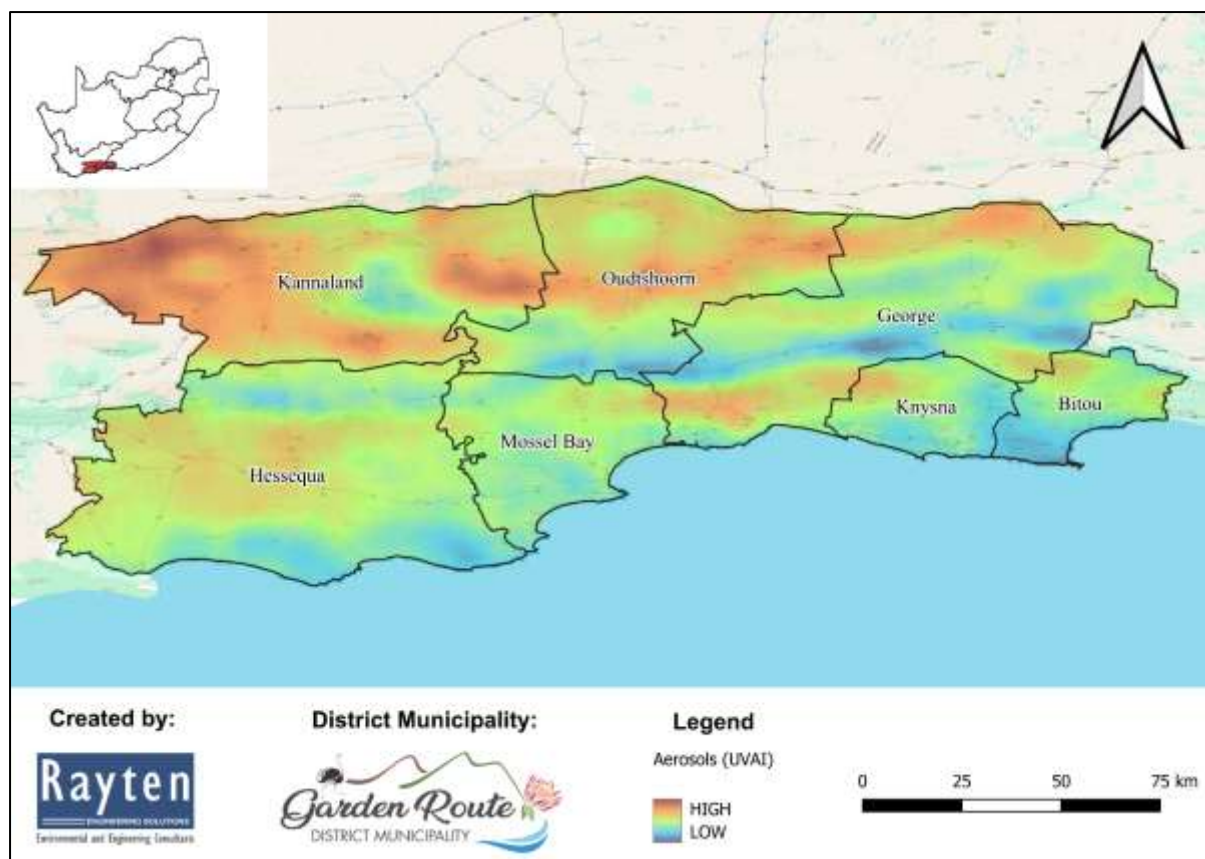
Figure 5-14: Air quality report map indicating concentrations of aerosols (UVAI) in the GRDM.
