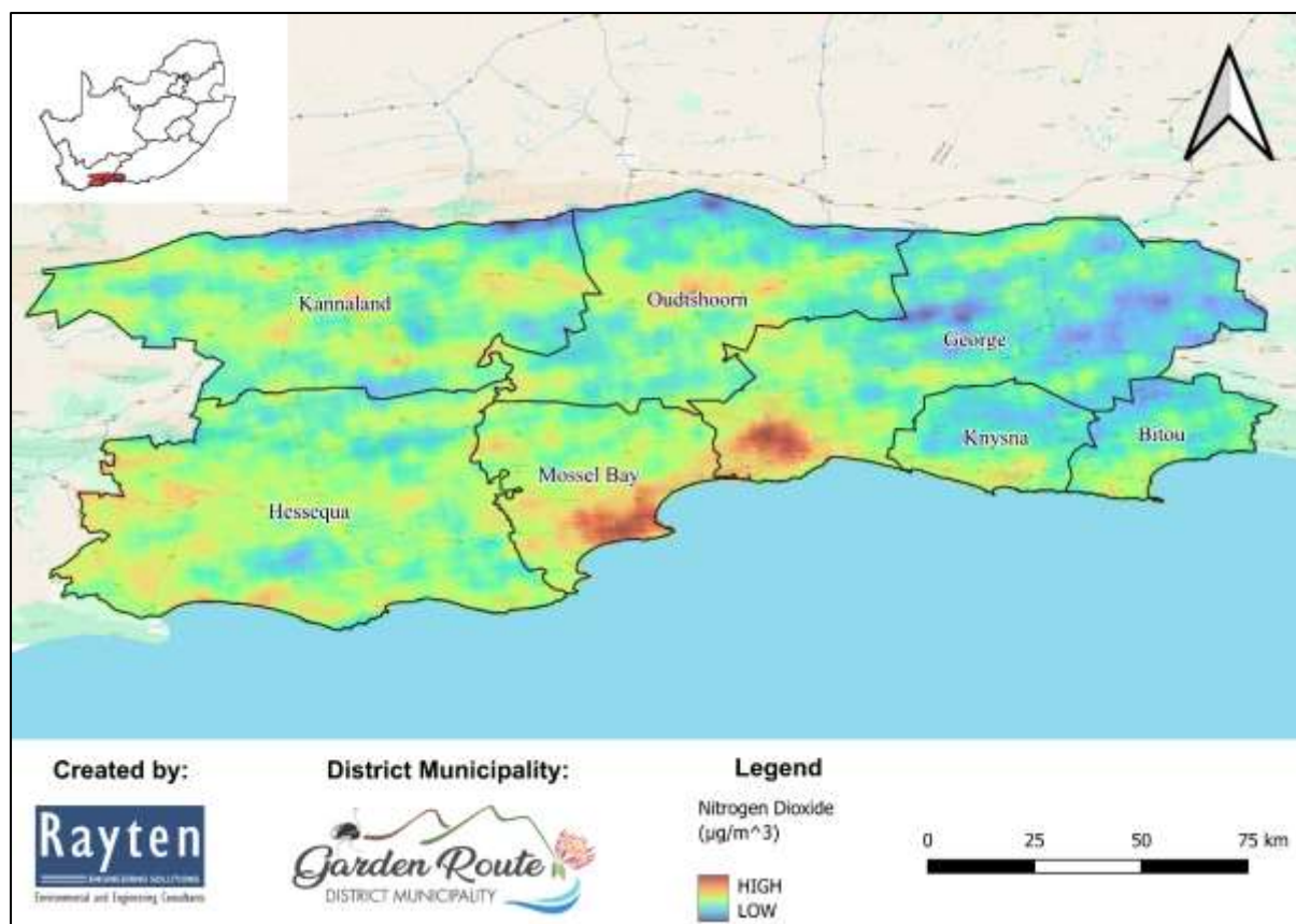
Figure 5-10: Air quality report map indicating concentrations of nitrogen dioxide ( \mu\text{g}/\text{m}^3 ) in the GRDM.
