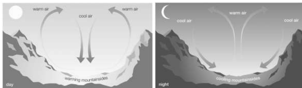
Figure 4-3: Air circulation in a valley illustrating anabatic (day) and katabatic (night) winds (Encyclopaedia Britannica, Inc. 2011).
