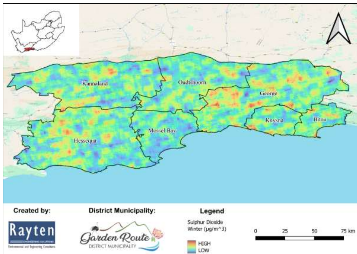
Figure 5-8: Air quality report map indicating concentrations of sulphur dioxide ( \mu\text{g}/\text{m}^3 ) in winter in the GRDM for each season.
