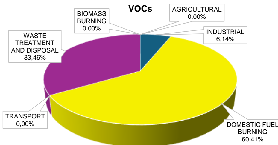
Figure 6-9: The contribution of emissions by sector of volatile organic compounds in the Bitou LM.
