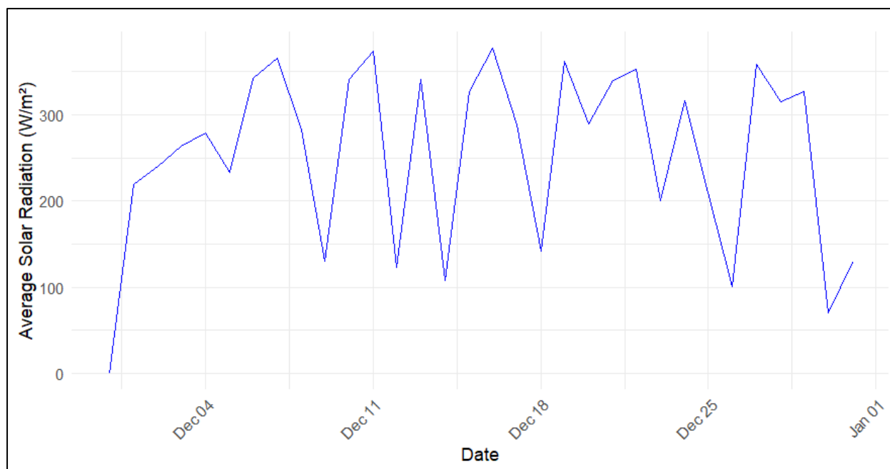
Figure 4-8: Solar radiation in the GRDM for the Summer months (excluding January and February) for 2023
