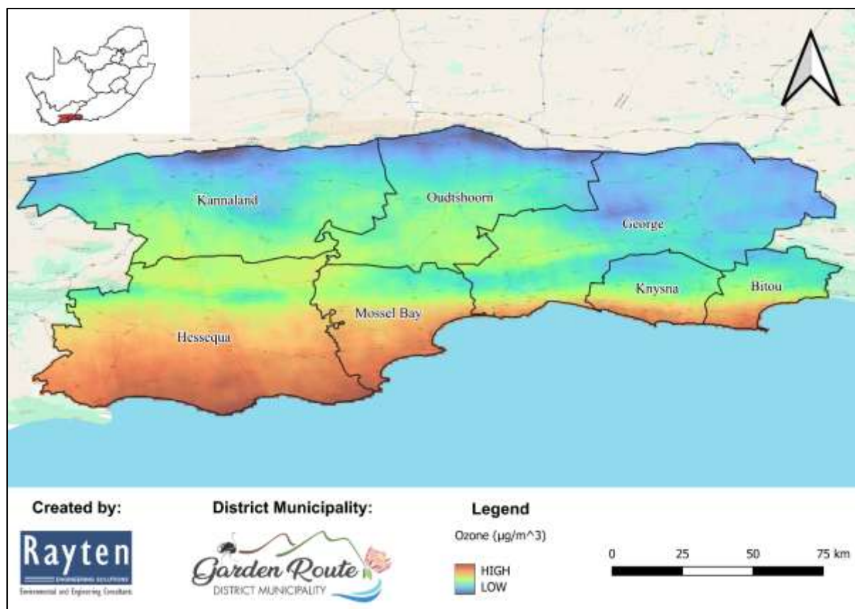
Figure 5-12: Air quality report map indicating concentrations of ozone ( \mu\text{g}/\text{m}^3 ) in the GRDM.
