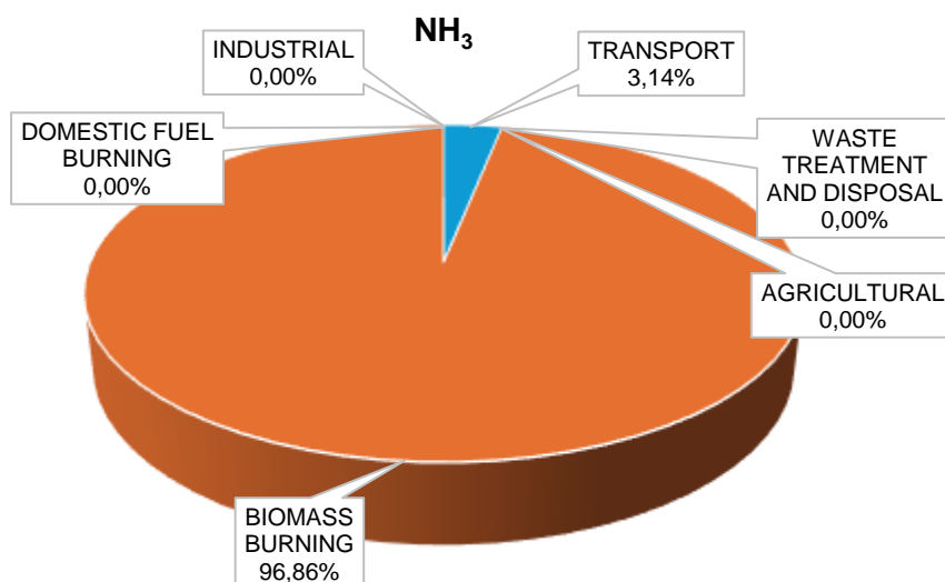
Figure 6-12: The contribution of emissions by sector of ammonia in the Bitou LM.
