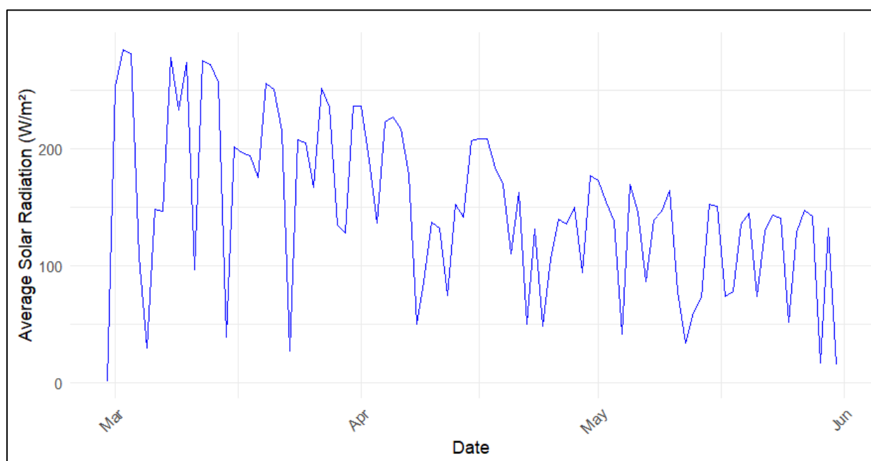
Figure 4-9: Solar radiation in the GRDM for the Autumn months for 2023.
