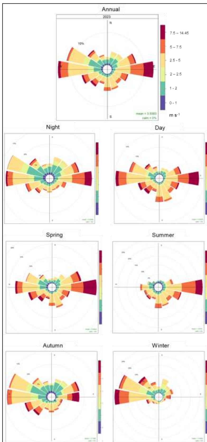
Figure 4-4: Wind roses to depict the wind strength, direction and frequency in the GRDM in 2023. Annual, day and night and seasonal wind roses are illustrated.
