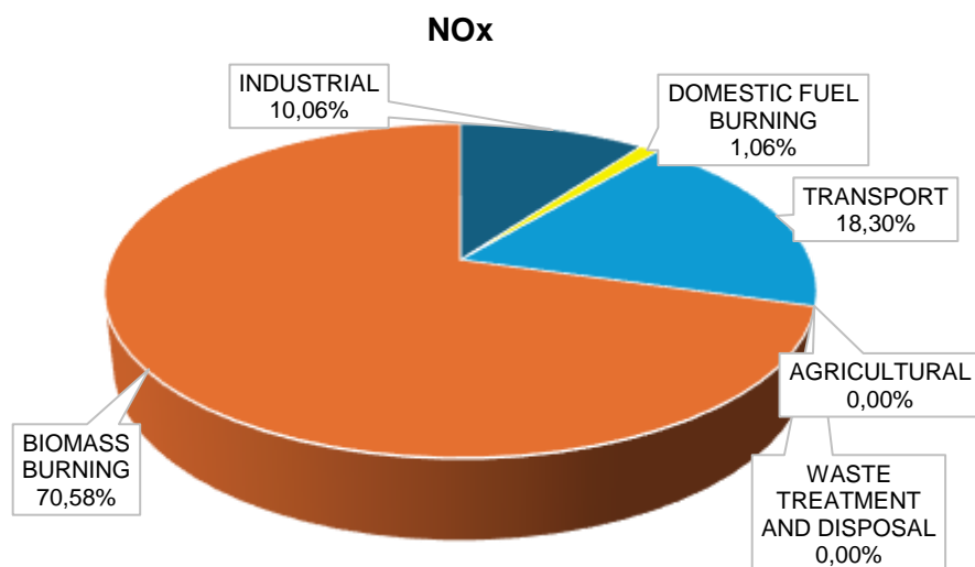
Figure 6-11: The contribution of emissions by sector of nitrogen oxides in the LM.
