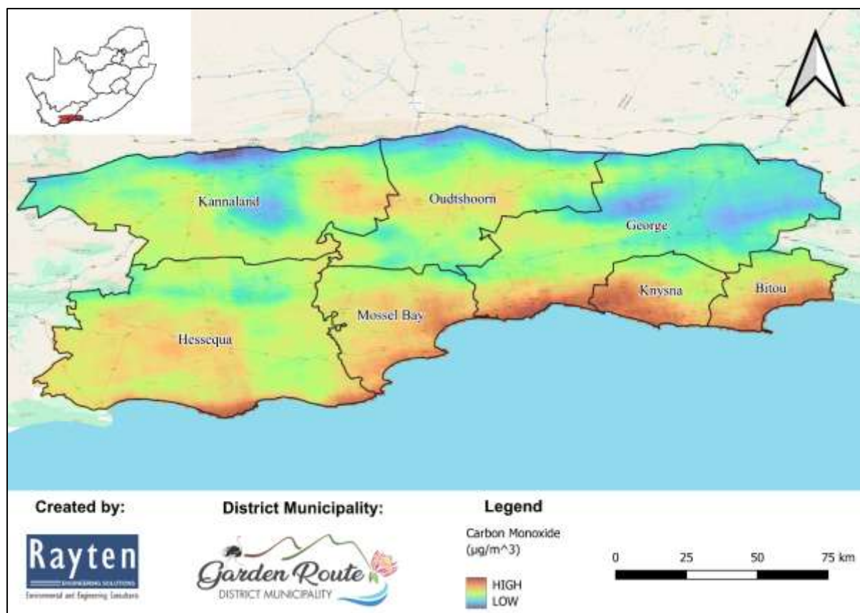
Figure 5-11: Air quality report map indicating concentrations of carbon monoxide ( \mu\text{g}/\text{m}^3 ) in the GRDM.
