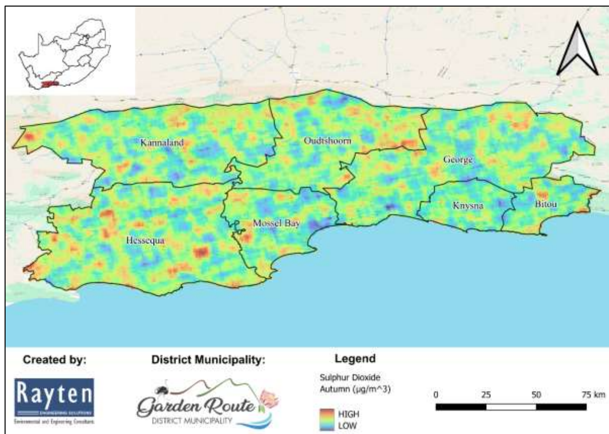
Figure 5-7: Air quality report map indicating concentrations of sulphur dioxide ( \mu\text{g}/\text{m}^3 ) in autumn in the GRDM for each season.
