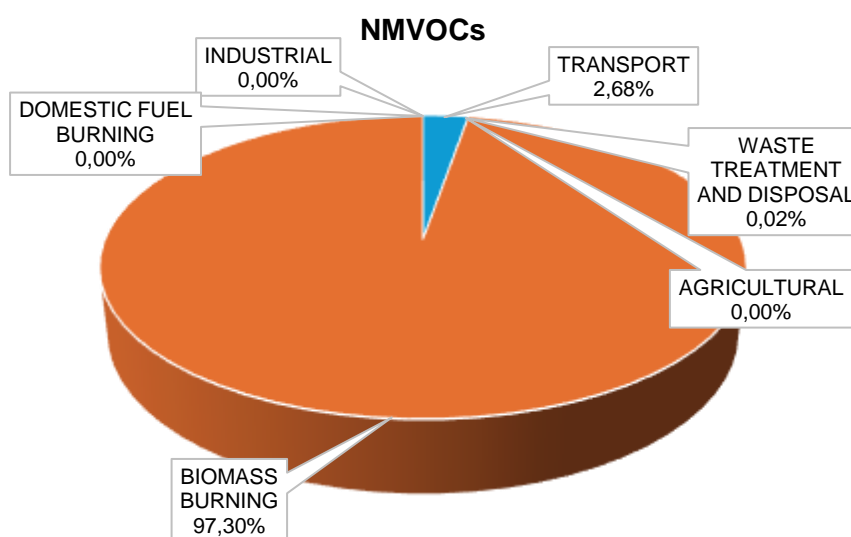
Figure 6-10: The contribution of emissions by sector of non-methane volatile organic compounds in the Bitou LM.
