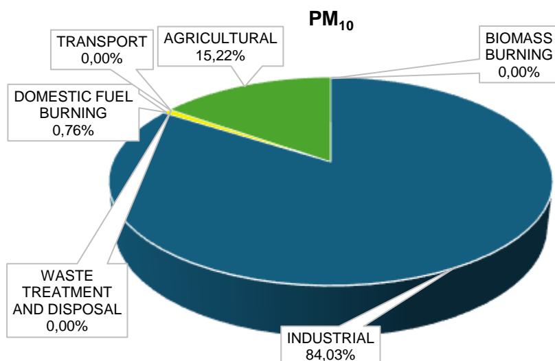
Figure 6-5: The contribution of emissions by sector of particulate matter with a diameter of 10 micrometres or less in the Bitou LM.
