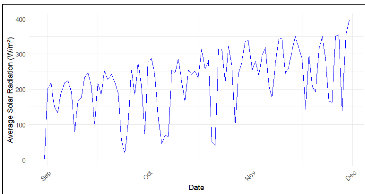
Figure 4-11: Solar radiation in the GRDM for the Spring months for 2023.
