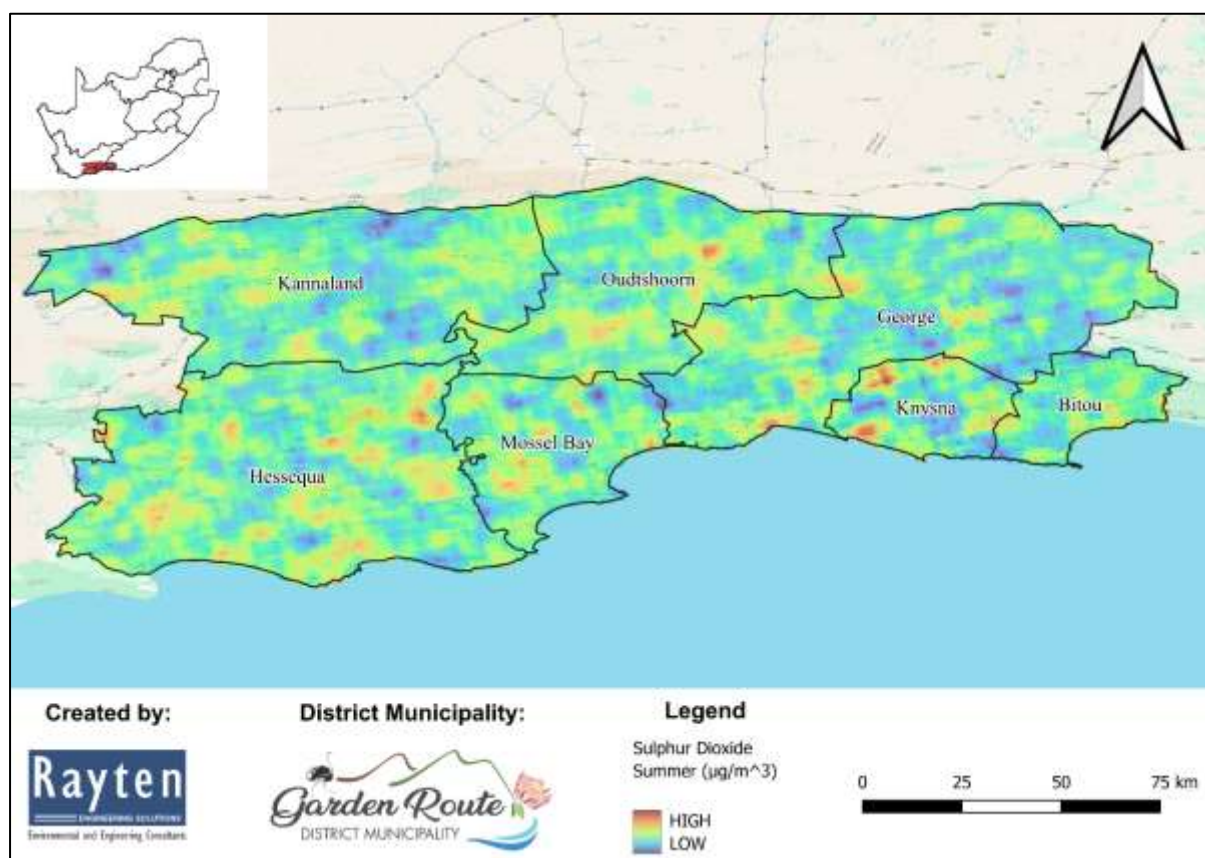
Figure 5-6: Air quality report map indicating concentrations of sulphur dioxide (µg/m 3 ) in summer in the GRDM for each season.
