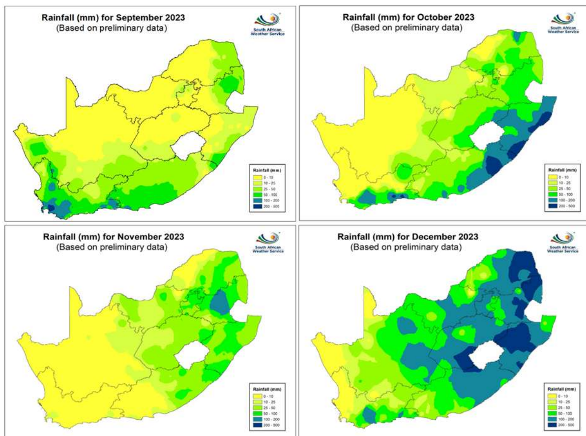
Figure 4-6: Rainfall in mm in South Africa for the year 2023. Key clarification: Bright Yellow = 0-10mm, Light Yellow = 10-25mm, Light Green = 25-50mm, Bright Green = 50-100mm, Light Blue = 100-200mm, Dark Blue = 200-500mm.
