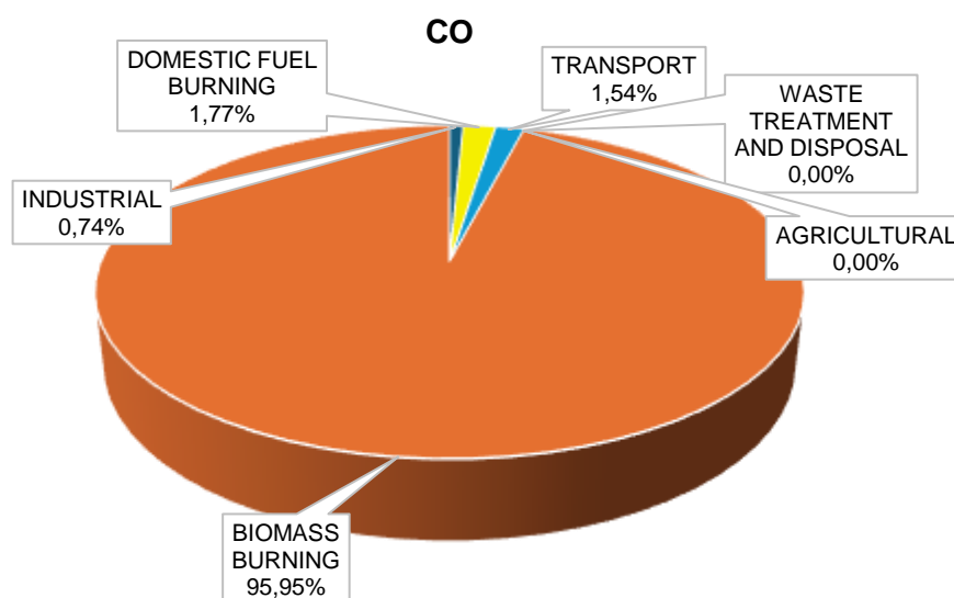
Figure 6-8: The contribution of emissions by sector of carbon monoxide in the Bitou LM.
