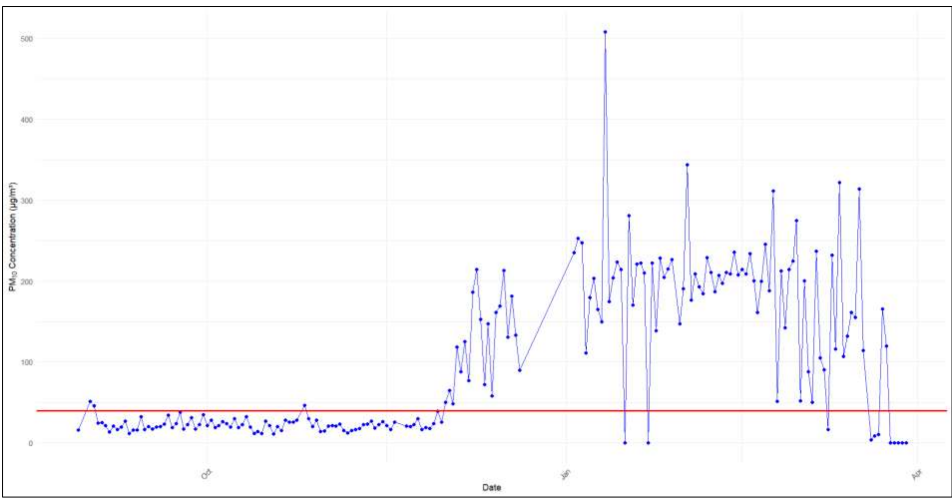
Figure 5-3: Concentration in \mu\text{g}/\text{m}^3 of \text{PM}_{10} as recorded by the Mossel Bay ambient air quality station from 2022 to 2024. The red dotted line represents the daily threshold as per the regulations set out in NAAQS.
