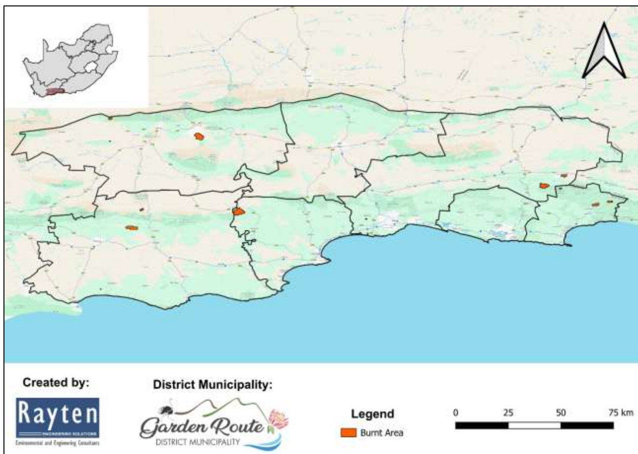
Figure 6-4: Map of the biomass burned in the GRDM from August 2023 to July 2024.
