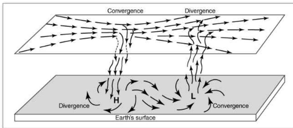
Figure 4-2: The relationship between horizontal and vertical motion in the troposphere (chegg.com).
