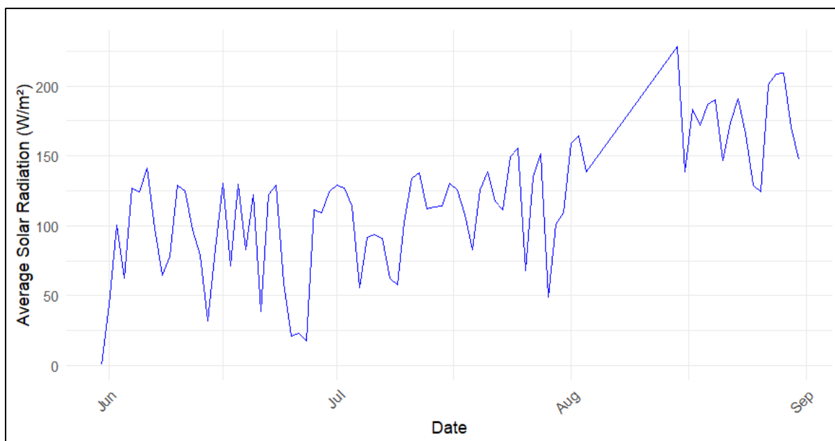
Figure 4-10: Solar radiation in the GRDM for the Winter months for 2023
