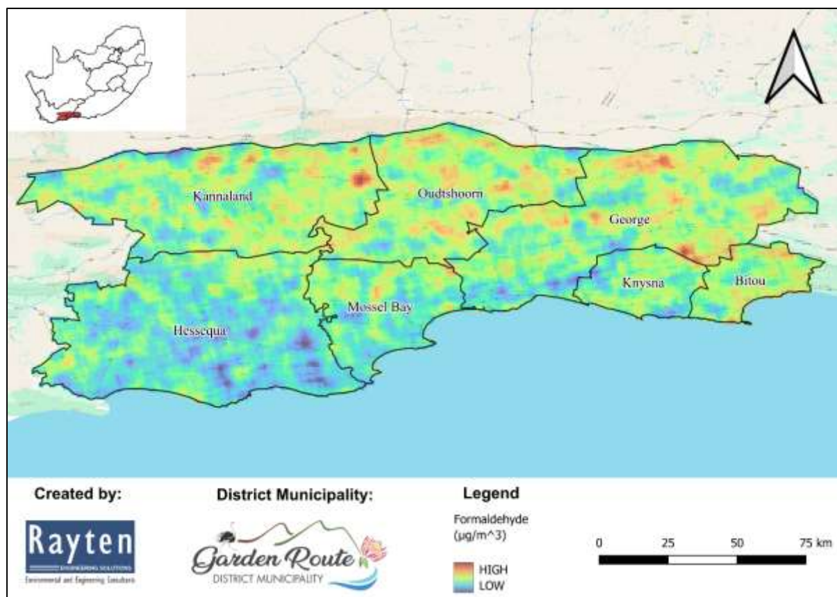
Figure 5-13: Air quality report map indicating concentrations of formaldehyde ( \mu\text{g}/\text{m}^3 ) in the GRDM.
