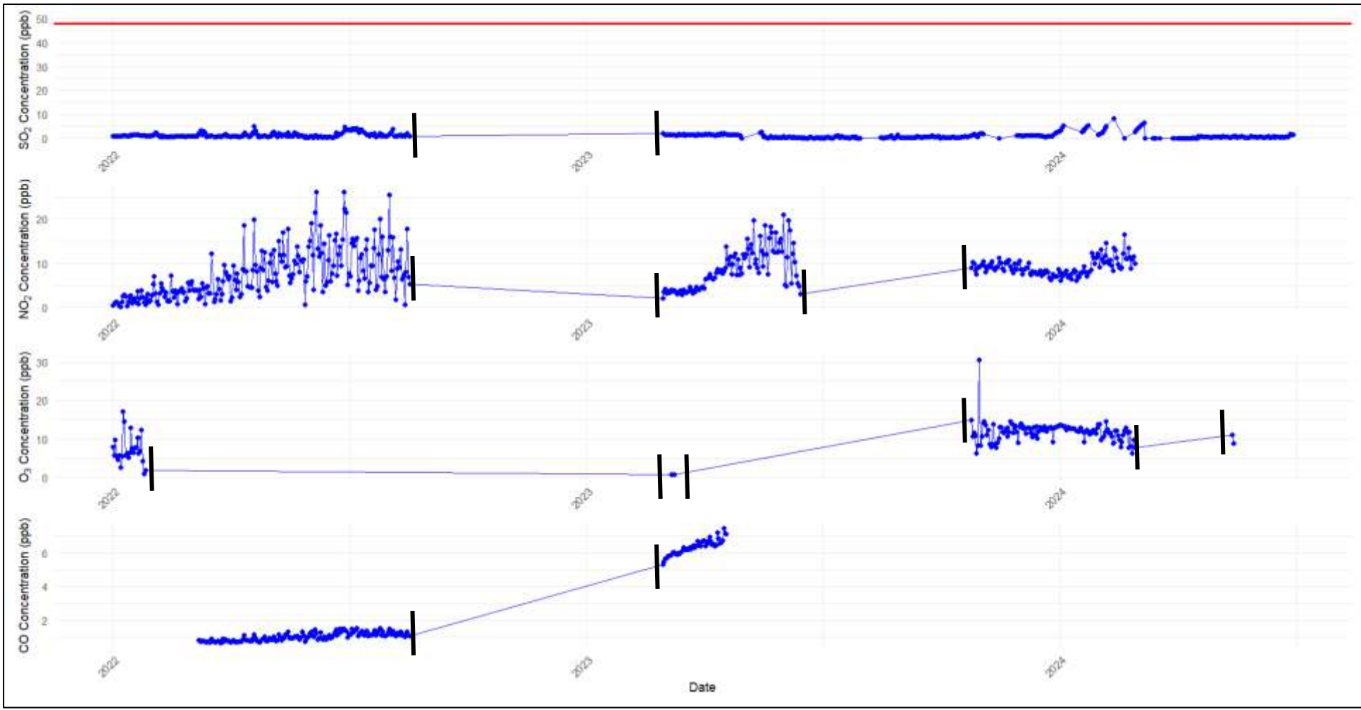
Figure 5-1: Concentration in ppb of SO 2 , NO 2 , O 3 and CO as recorded by the George ambient air quality station from 2022 to 2024. The red dotted line represents the daily threshold for SO 2 as per the regulations set out in NAAQS.
